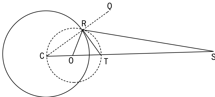
Alhazen's idea of the formation of the rainbow.
